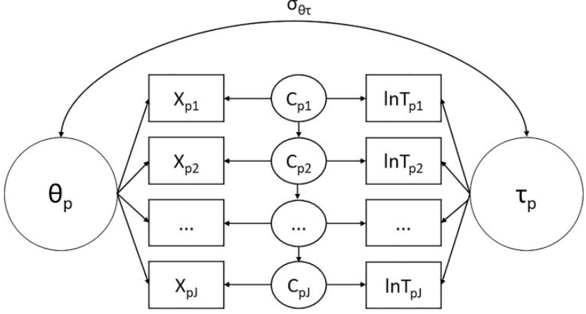
FIGURE 1. Markov-dependent item states model.
