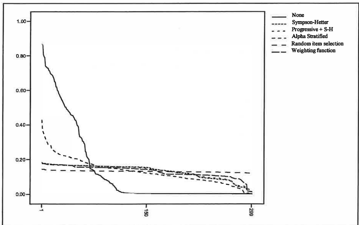
Figure 3. Observed exposure rates for different exposure control problems.
