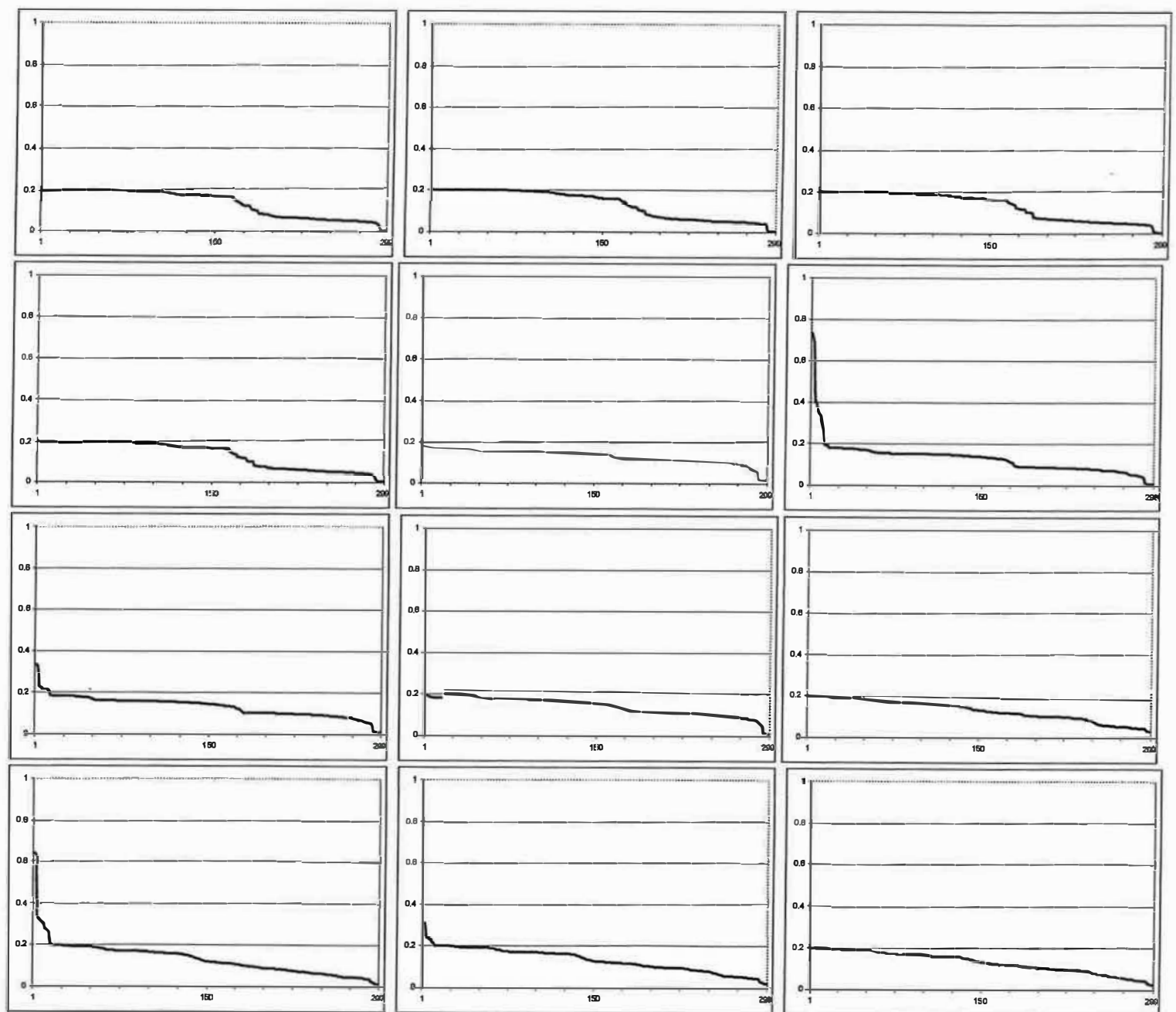
Figure 2. Observed exposure for different settings of the multiple objective exposure control method r_{\max}=0.20 .
